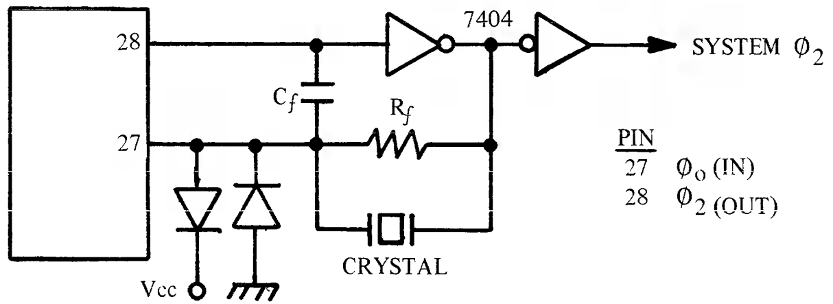
MCS6503,4,5 Series Mode Crystal Controlled Oscillator
